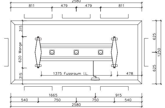
Meeting table C 20 and C 21 / C 43 Power box for meeting table
