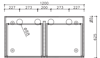
Meeting table C 20 and C 21 / C 42 Cable outlet
