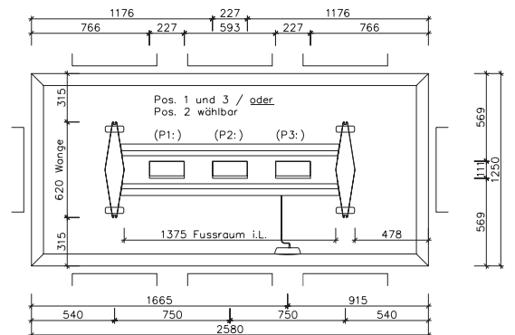
Meeting table C 20 and C 21 / C 43 Power box for meeting table
